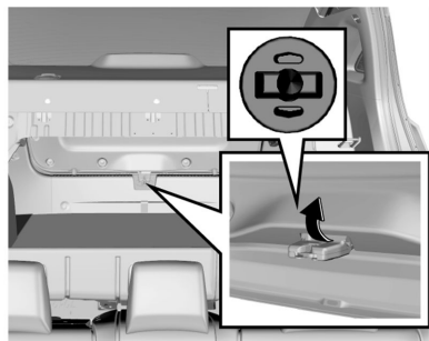
Notchback
